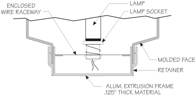
Frame Cross Section View
